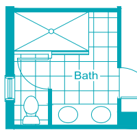
Master Bath Double Sink Option
